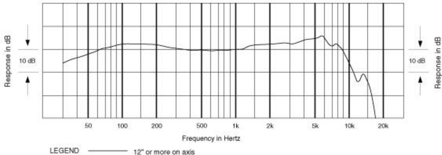
Frequency Response
