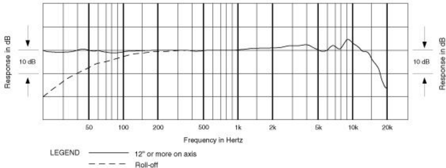
Frequency Response
