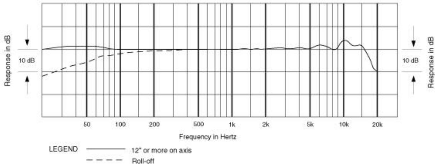
Frequency Response
